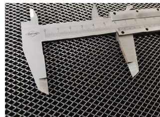
Small holes steel expanded mesh is good material for air filters
