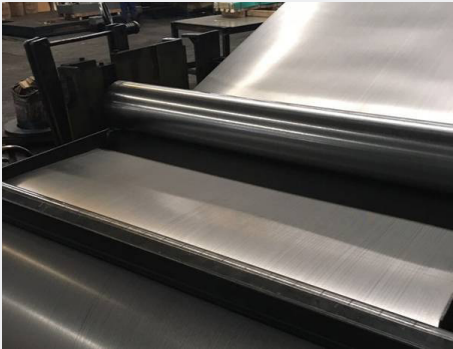
MHPM-04: 0.4mm stainless steel 316L Micro Hole Perforated Metal Plate
