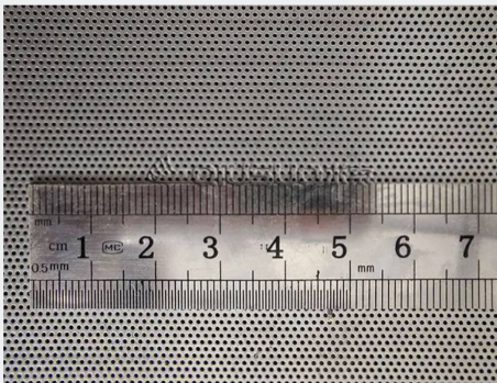
MHPM-12: 0.6mm hole x 1.2mm pitch stainless steel perforated sheets
