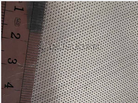
MHPM-11: 0.4mm hole x 1.2mm pitch stainless steel perforated sheets
